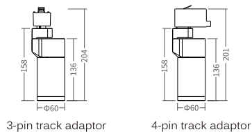
3-pin track adaptor
