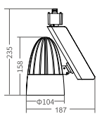
3-pin track adaptor
