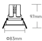
DM060-DF62RF02N / DM060P-DF62RF02N
